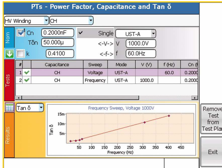
Figure 13 - "PTs – Power Factor, Capacitance and Tan \delta " page
