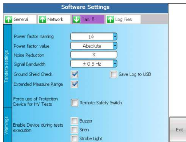
Figure 14 - "PTs – Software settings, Tan \delta " page
