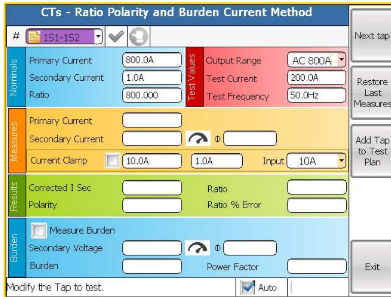
Figure 12 - "CTs – Ratio Polarity and Burden Current Method" page
