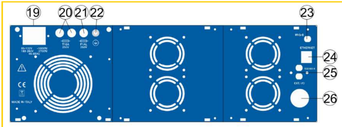
Figure 2 - Rear panel
